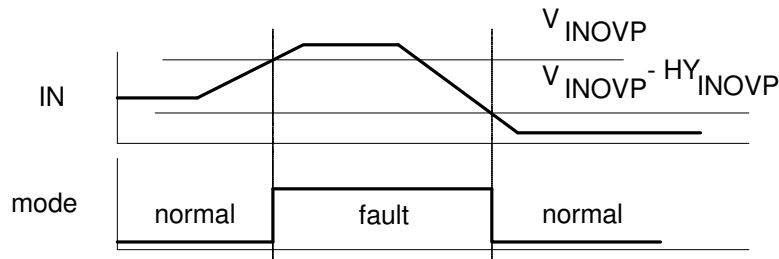
Figure 5 - Output over voltage Protection
