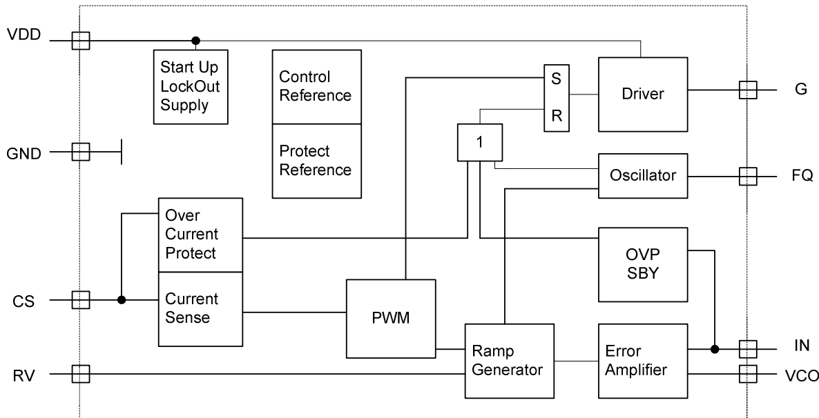
Figure 1 - Block diagram
