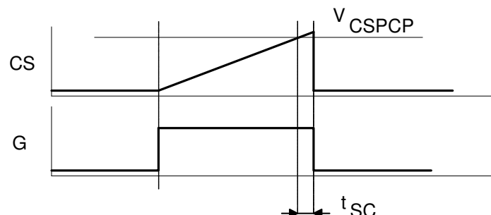
Figure 7 - Peak current limit protection
